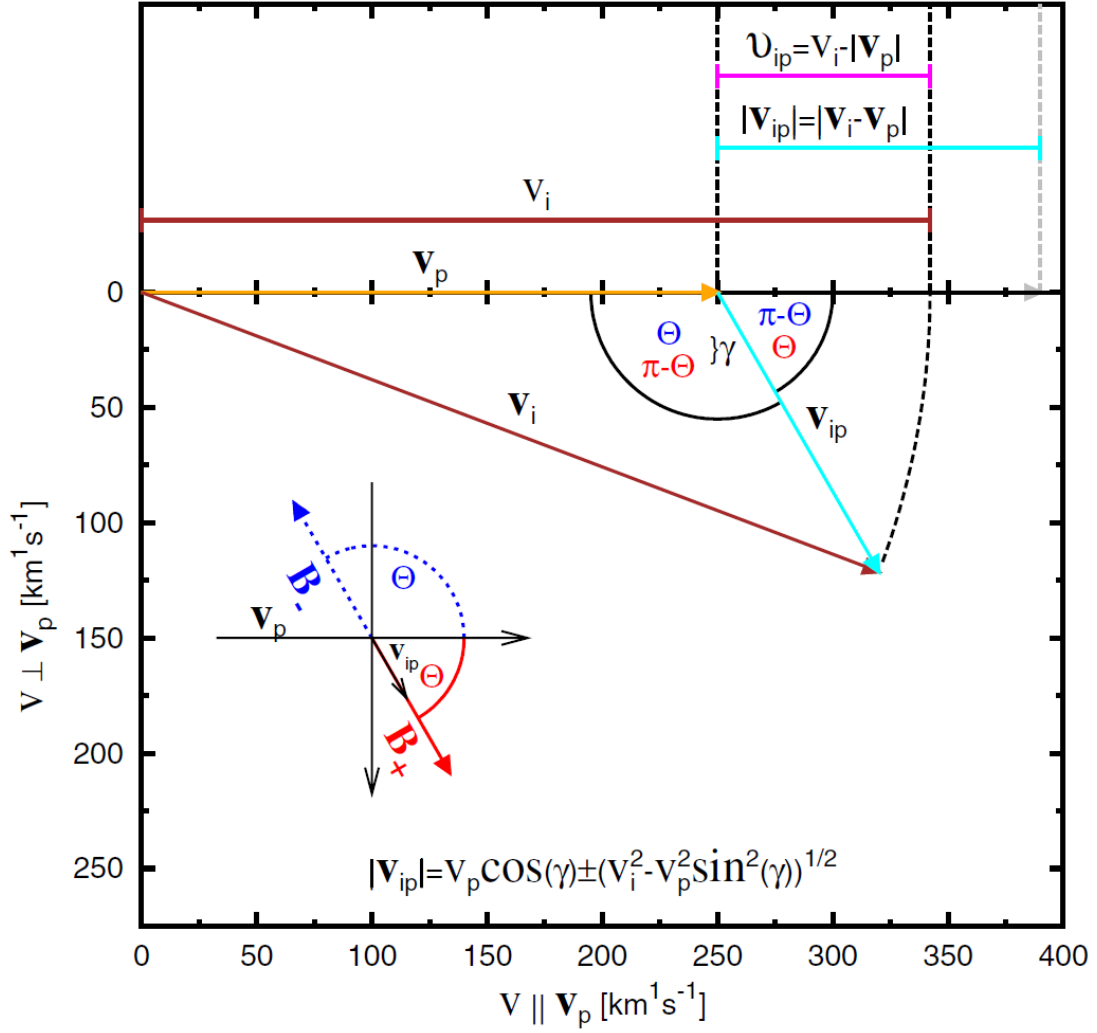
FIGURE 2.13: Measurement geometry for solar wind heavy ions (brown vector \mathbf{v}_i ) and protons (yellow vector \mathbf{v}_p ) in two-dimensional velocity space ( v_{\parallel}, v_{\perp} ) in the ecliptic plane. Both PM and CTOF measure the absolute value of the ion speed and not the full velocity vector. Therefore, the magnitude of the differential velocity \mathbf{v}_{ip} (also called differential speed \Delta v = v_{ip} ) which is oriented along the in-situ magnetic field, is systematically underestimated as v_{ip} = |\mathbf{v}_i| - |\mathbf{v}_p| (pink length bar) instead of v_{ip} = |\mathbf{v}_i - \mathbf{v}_p| (cyan length bar). If the in-situ B-field angle \theta is measured simultaneously with the particles the true differential speed v_{ip} can be reconstructed from the combination of both measurements after Eq. ?. Unfortunately, in the case of SOHO there are no magnetic field measurements conducted on the spacecraft, so that we can only apply a mean correction to the differential speed assuming a mean magnetic field angle of 45^\circ in the ecliptic plane corresponding to the Parker angle. The Figure is taken from [?] illustrating the measurements of solar wind ions at L1 with ACE/SWICS but is equivalently valid for our SOHO measurements. Also note, that the same geometrical relations between the shown ion velocities apply when we assume that the heavy ions flow approximately radially outwards from the Sun and instead the proton velocity shows a small deviation from the radial direction, as it is often observed for the case of alfvénic waves that are carried by the protons while the heavy ions surf these waves (see subsection 1.?)
