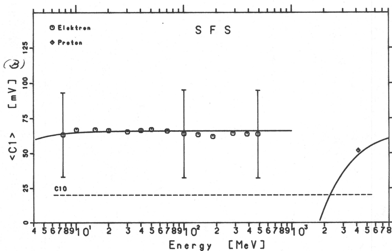
Figure 4-5 Peak location and width of the C1 - Cerenkov signal for (a) the SFM and (b) the SFS detector as a function of electron energy
