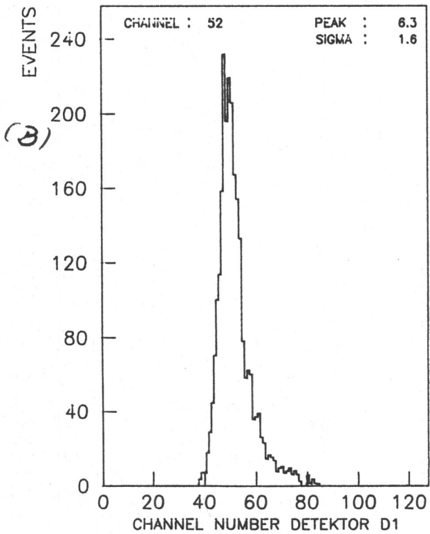
Figure 4-4 Pulse height distribution of the SFS detectors D1 and D2 for (a) 7.5 MeV electrons and (b) 185 MeV electrons
