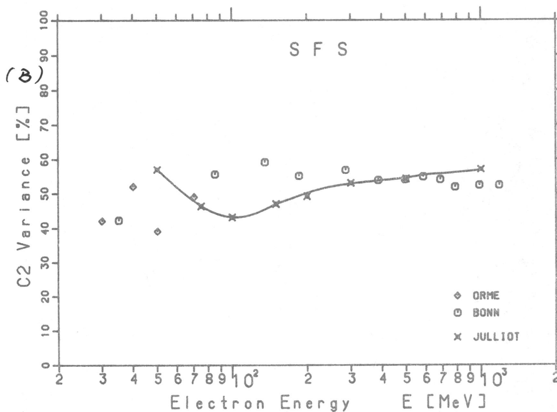
Figure 4-15 Variance of the pulse height distributions in C2 for penetration mode electrons as a function of energy for the SFM (a) and the SFS (b)
