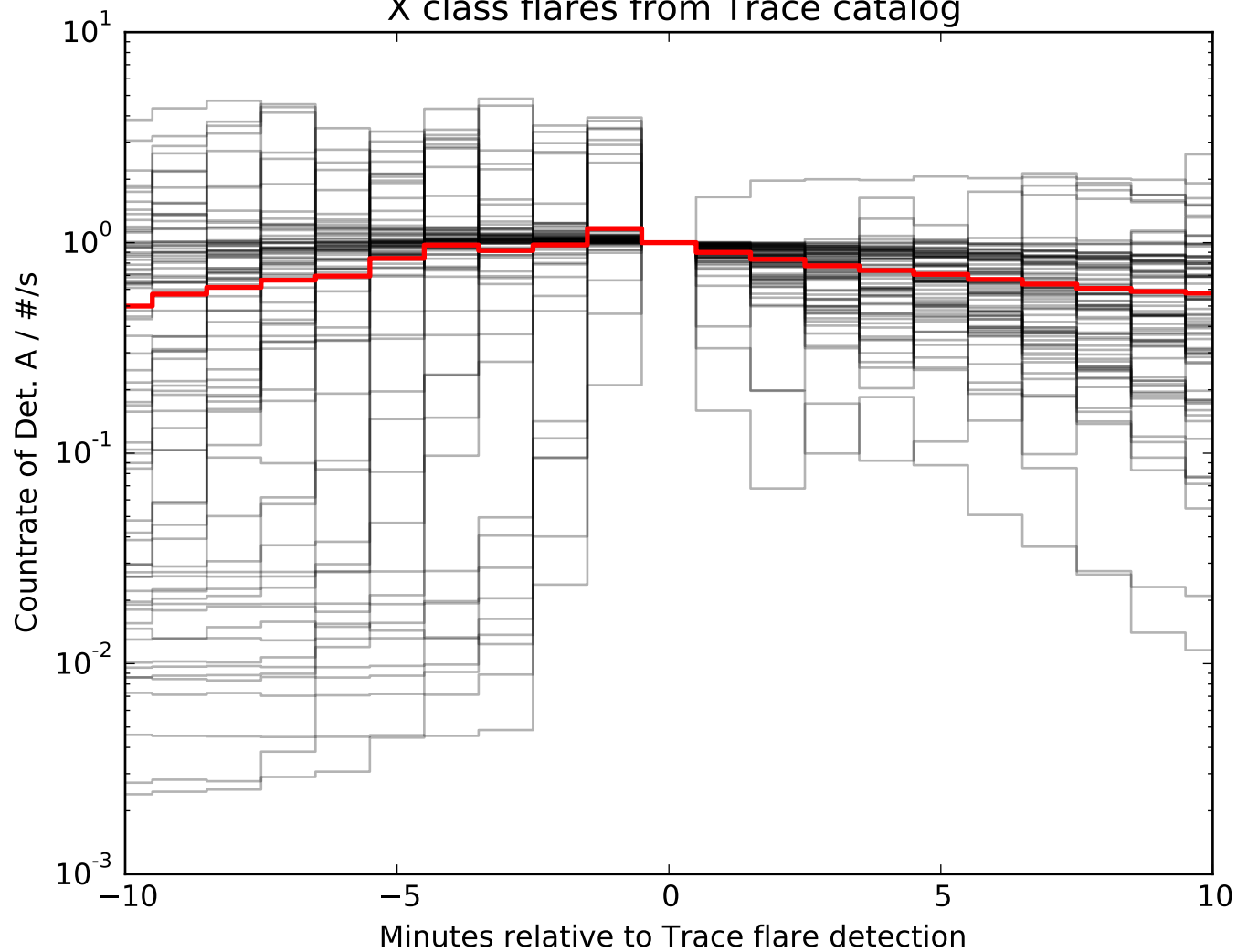
X class flares from Trace catalog
