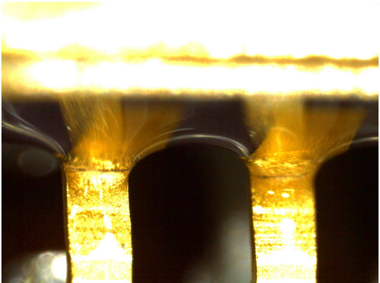
Abb 6 Crack on Pin 1 &2 at IC301 detail 01
