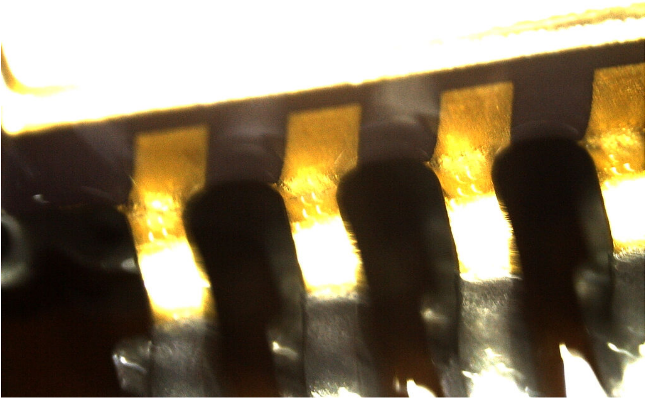
Abb 5 Crack on Pin 1 & at IC301
