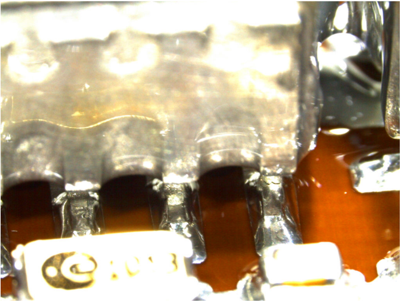
Abb 3 Crack at Capacitor C309
