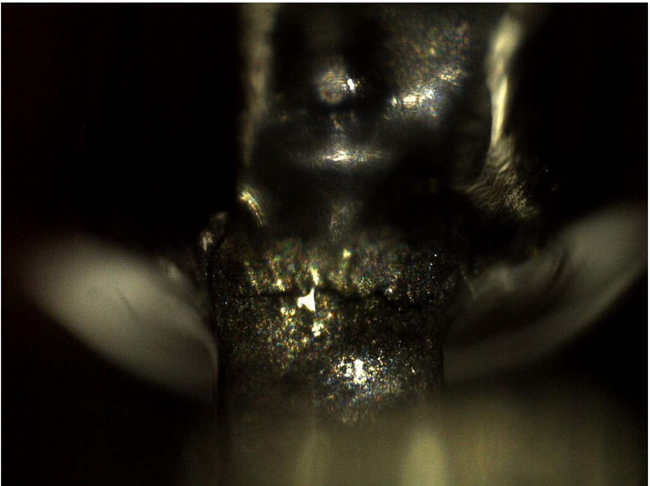
Abb 8 Crack at Capacitor C302
