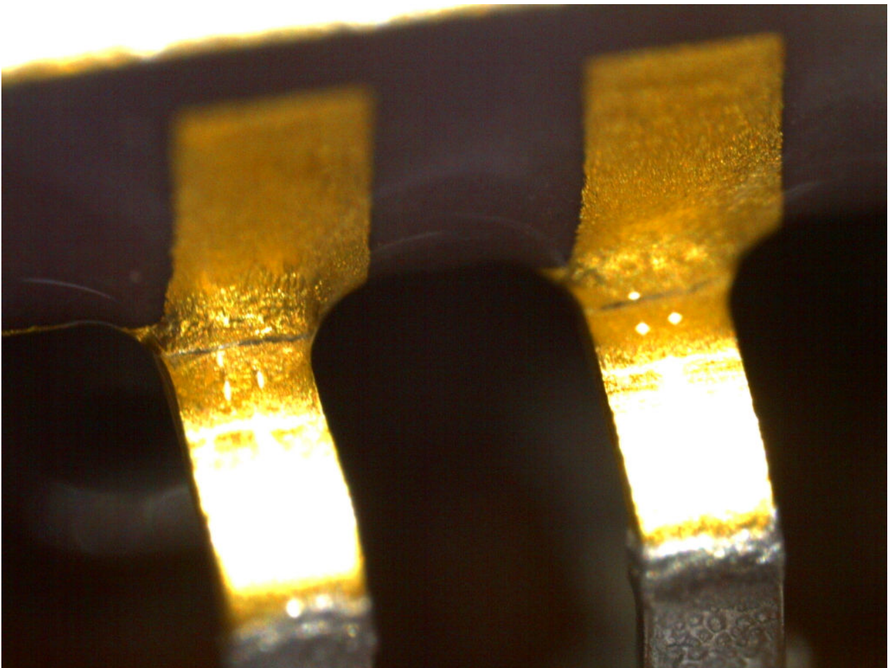
Abb 7 Crack on Pin 1 & 2 at IC301 detail 02
