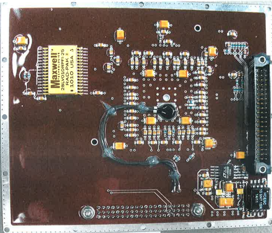
Solar Orbiter - CAU EPT_HET Digital Board PQM LS
