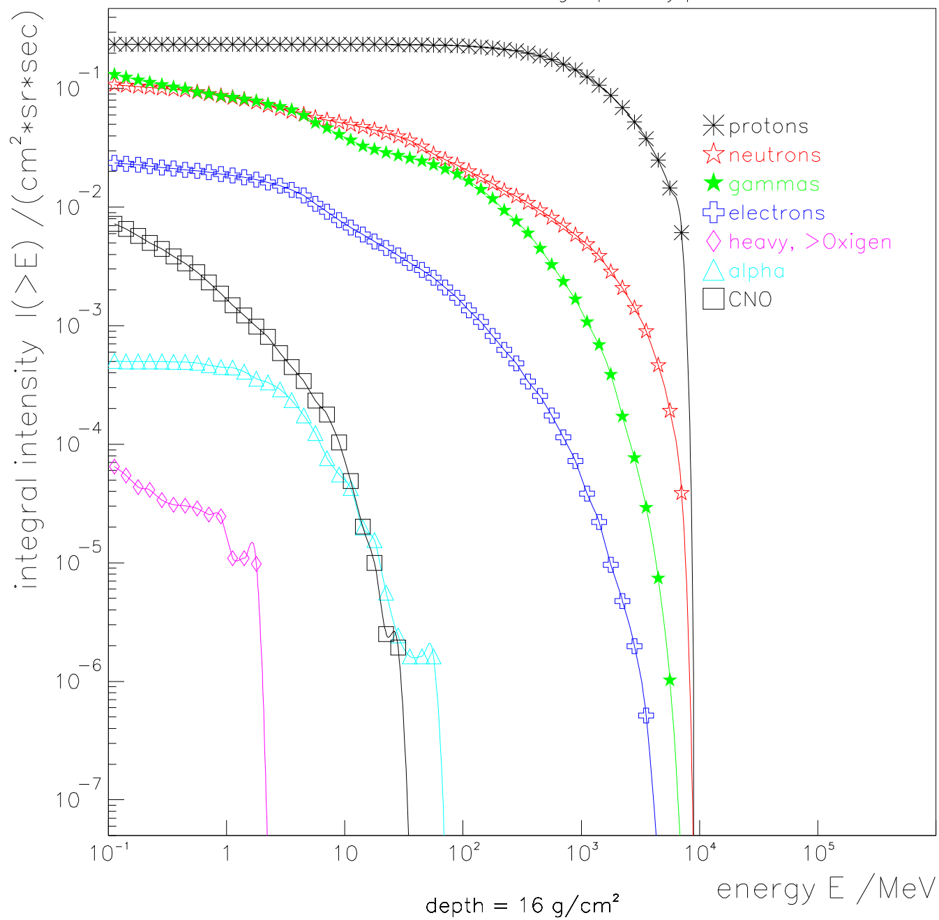
ICRC 22, Badhwar S.646 fig.2 primary protons
