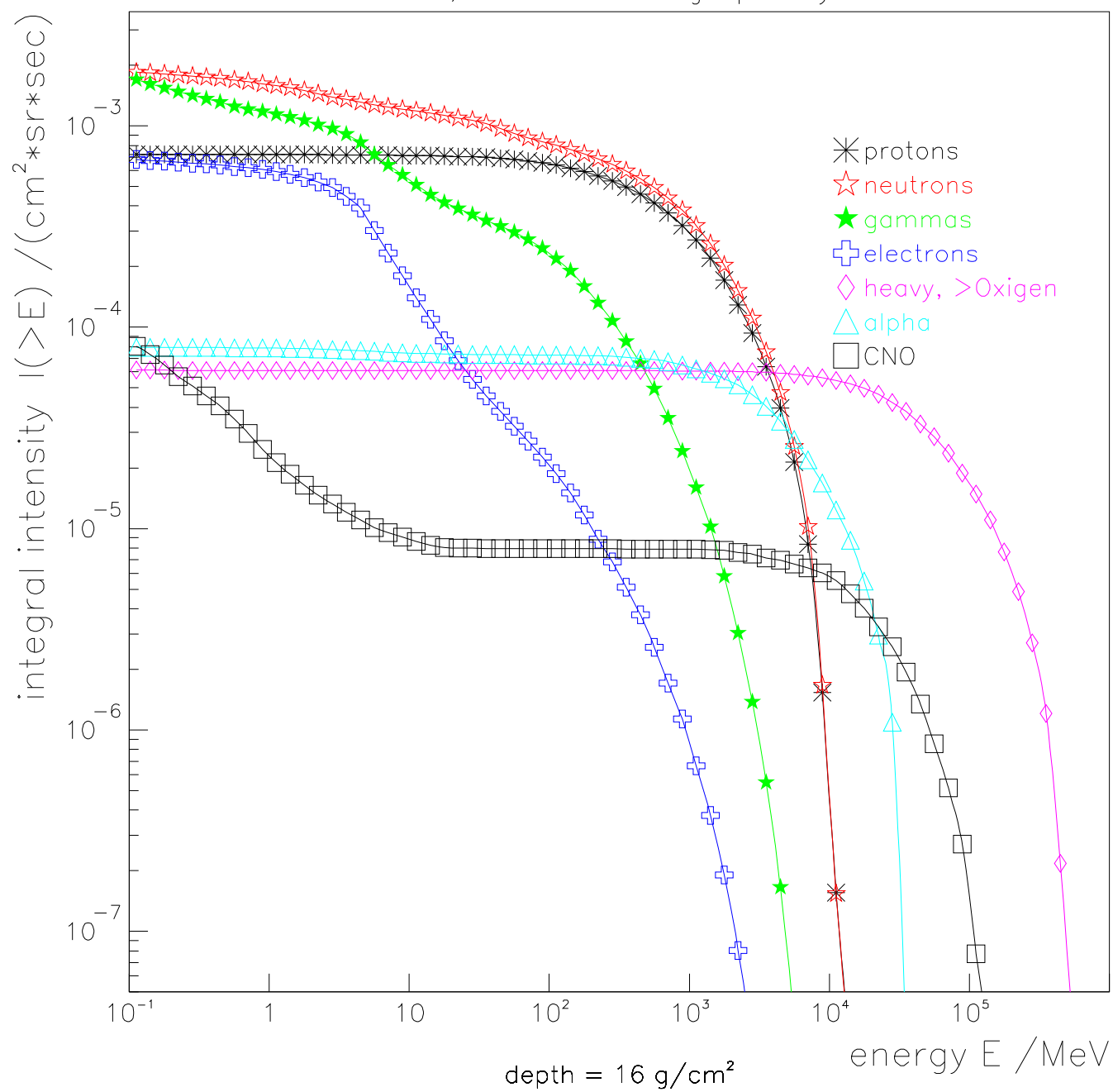
ICRC 22, Badhwar S.646 fig.4 primary iron
