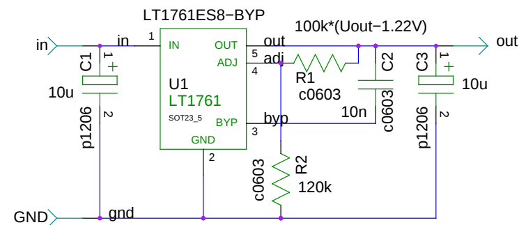
Low noise positive LDO regulator
