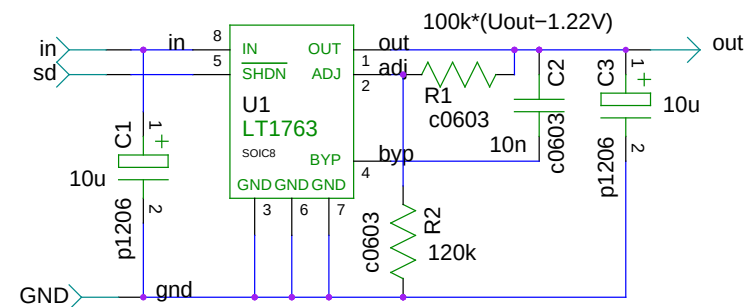
Low noise positive LDO regulator
