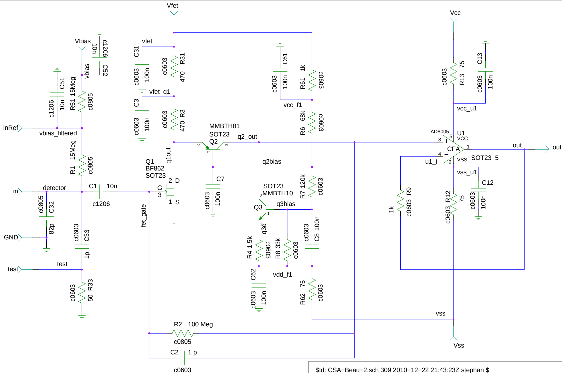
Common base stage with current source type Charge Sensitive Amplifier
