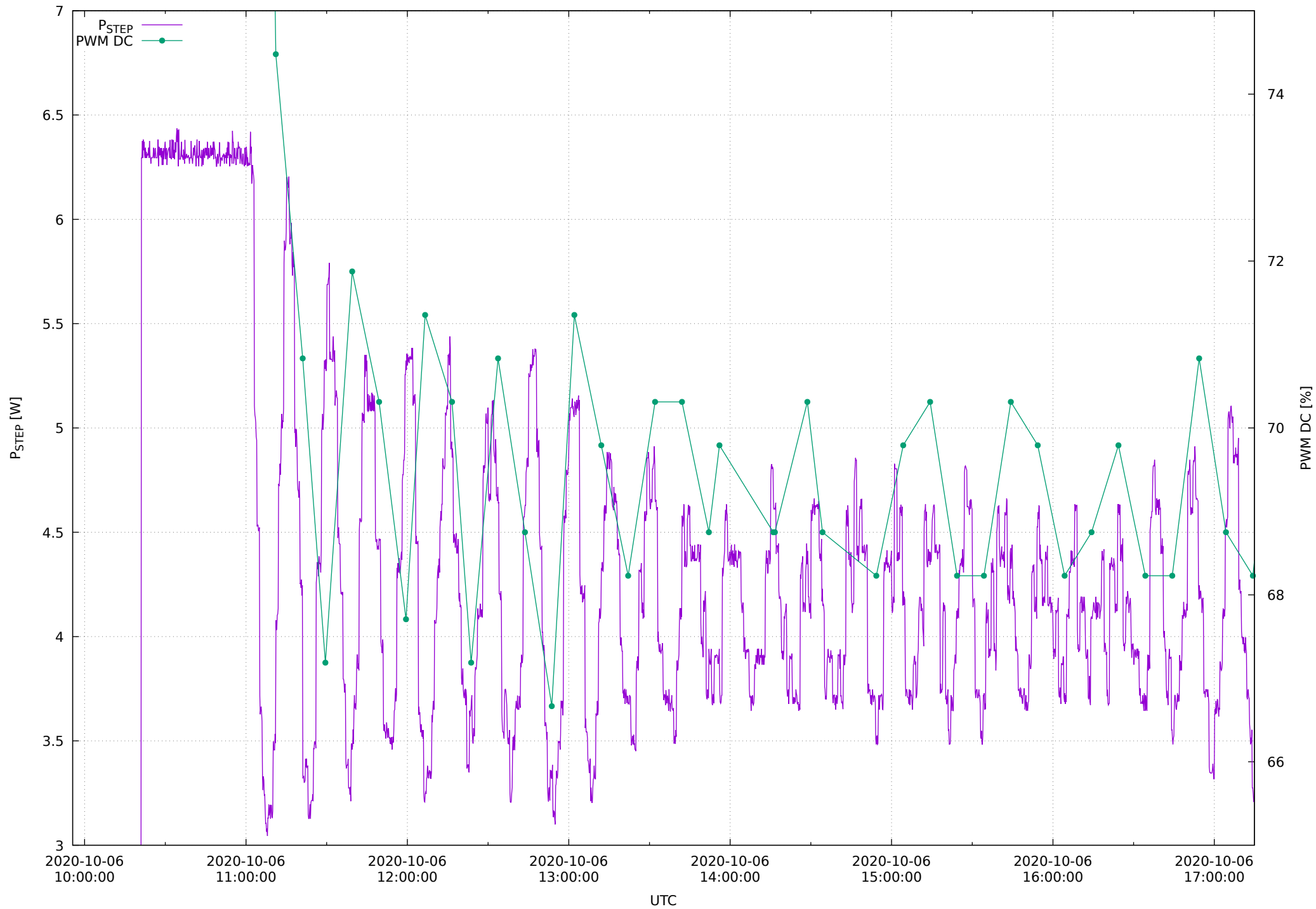
STEP Operational Heater, October 2020
